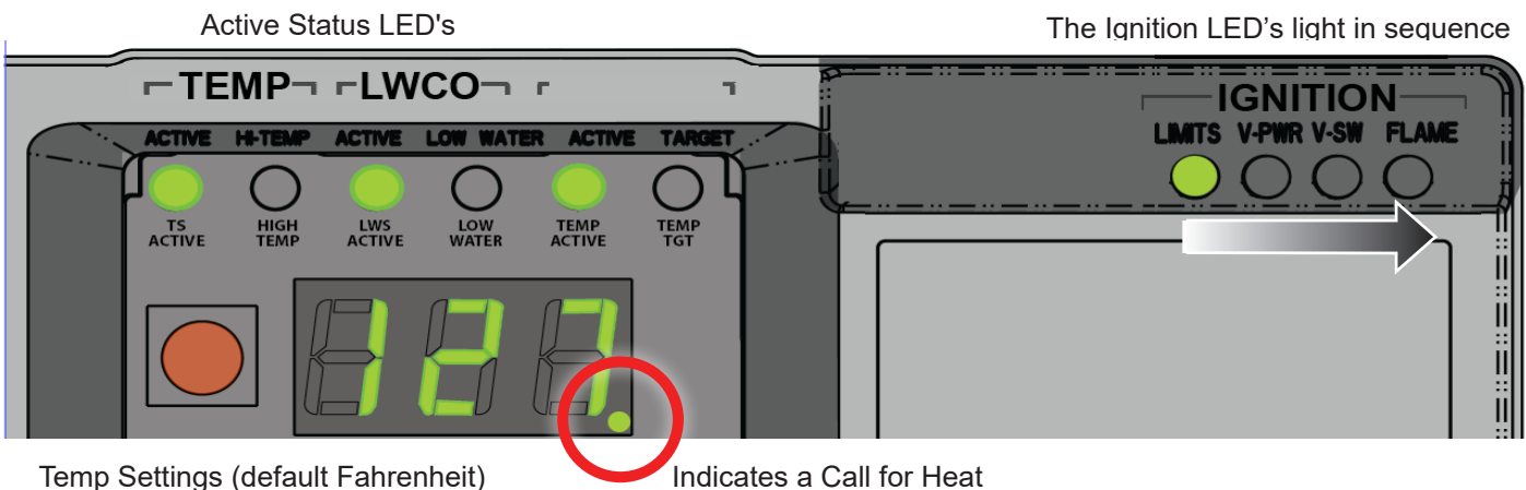
Figure 1. The indicator lights on the Digital Dashboard
