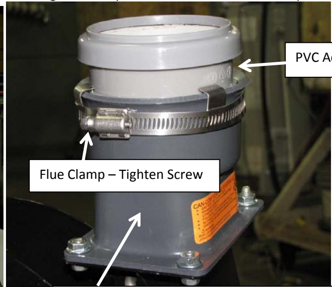
Commercial Power Direct Vent Exhaust Outlet Adapter
