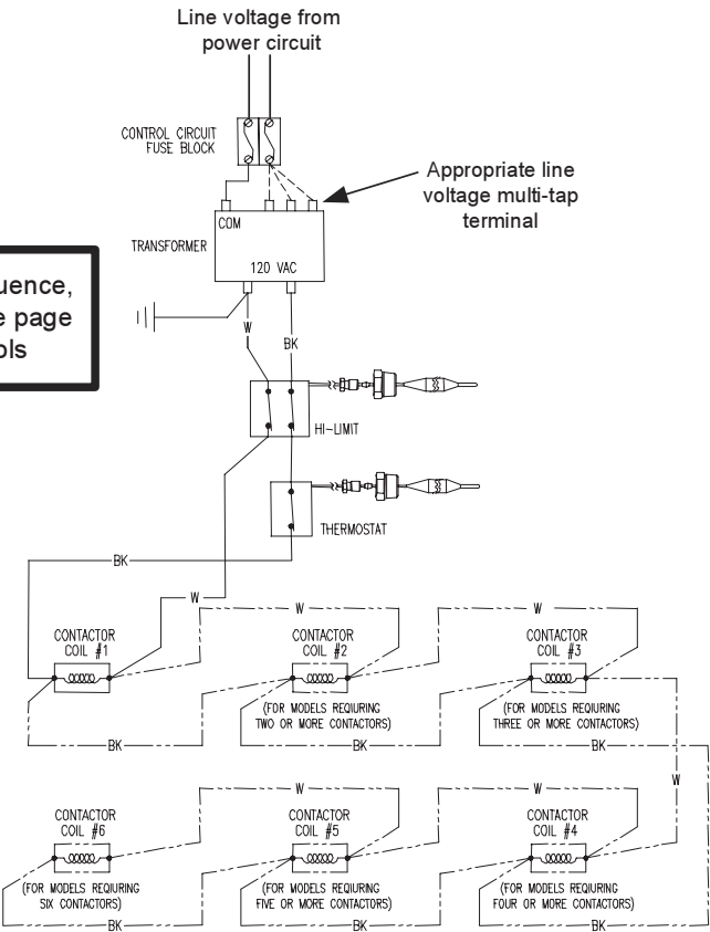
Control Circuit Wire Diagram
