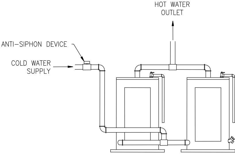
Figure 4A (Dual Water Heater Installation) 50A, 80A, 120A
